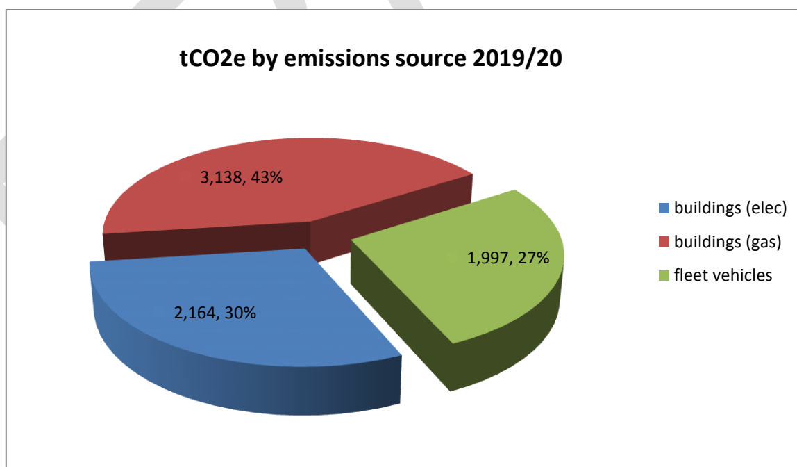
Figure 4: Oxford City Council's emissions by source 2019/20
